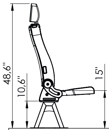
Single legs Flip-up
