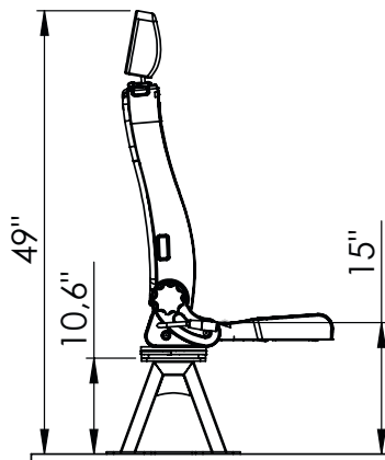
Single legs Tip&Fold
